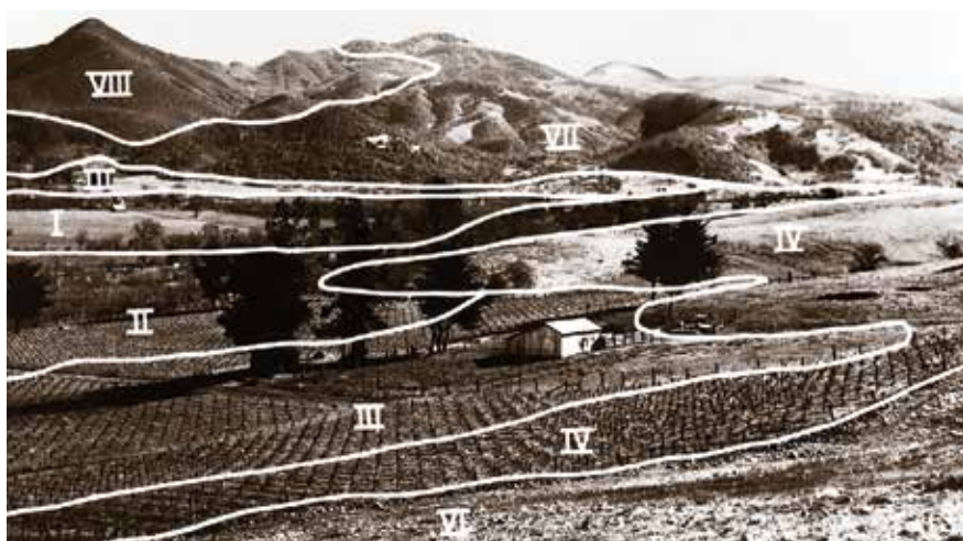
Land-capability classification
