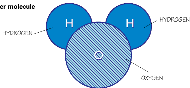
Water molecule
